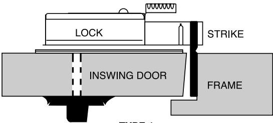
TYPE 1 Part# 114003
